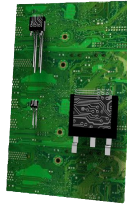
Condenser 100uf Condenser 0.1uf Regulator LM7805
